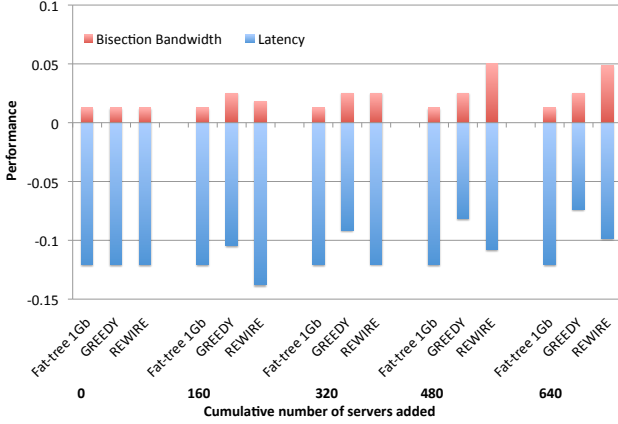
Fig. 4: Results of iteratively expanding the SCS data center.
