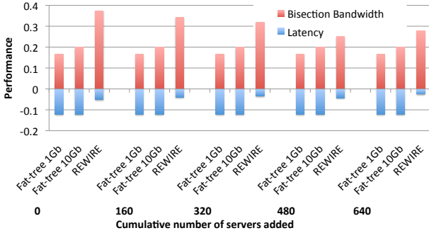
Fig. 5: Results of iteratively expanding a greenfield network.
